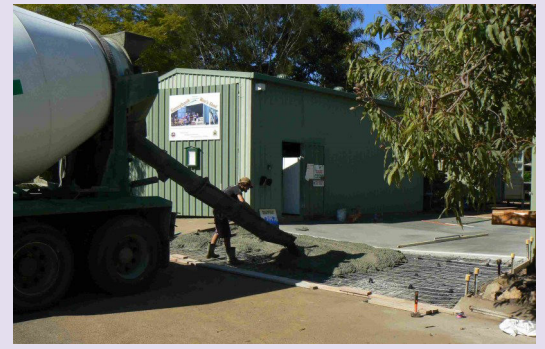
6. Finish off the area between the car park and the slab.
